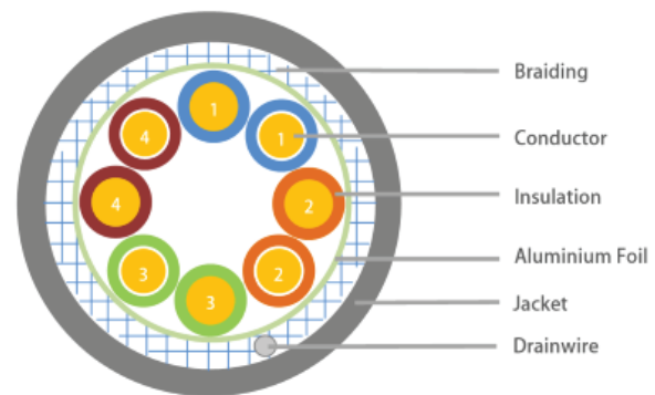
illustration for 4 pairs cable
