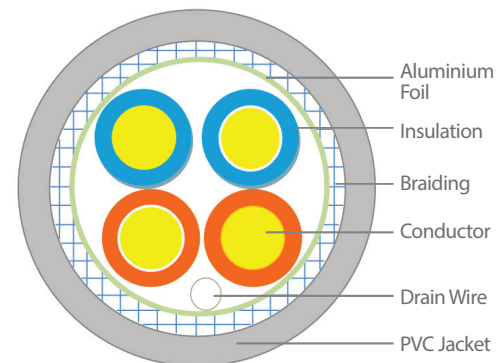
illustration for 4 pairs cable
